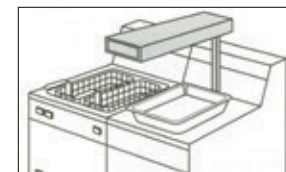
GRFS, GRFSL, GRFSC, GRFSC-18 with swing-away post mount and cord with plug
