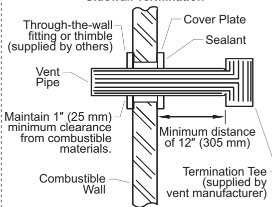
Typical Through-the-Wall Venting
