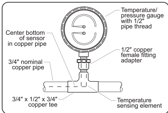
Alternate Temperature/Pressure Gauge Installation
