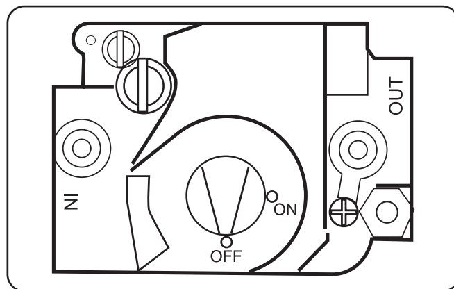
Gas Valve—Top View
