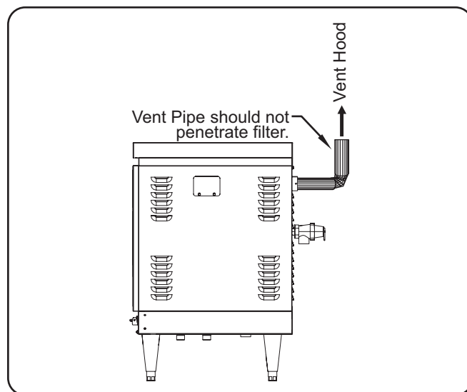
Venting Through Typical Exhaust System
