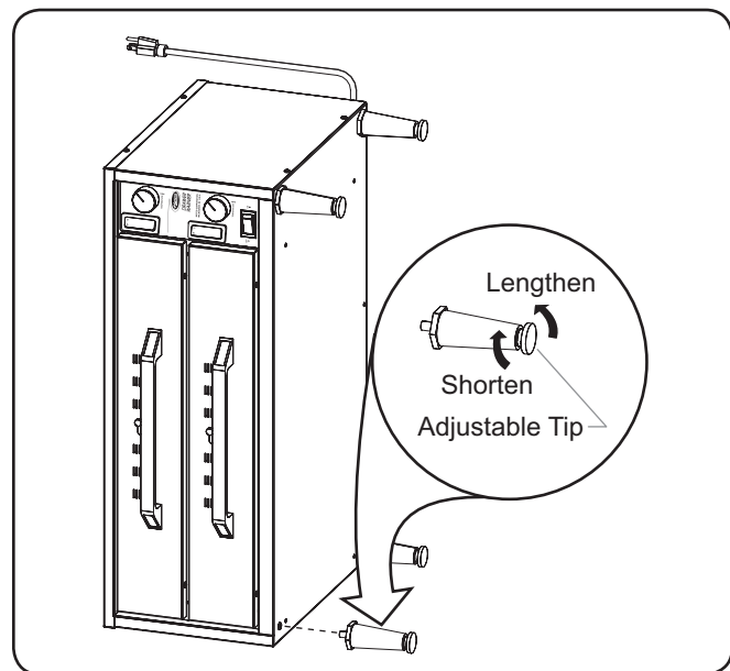
Leg Installation
