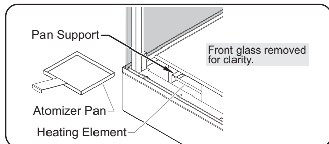
Atomizer Pan Location (IHDCH-45 shown)
