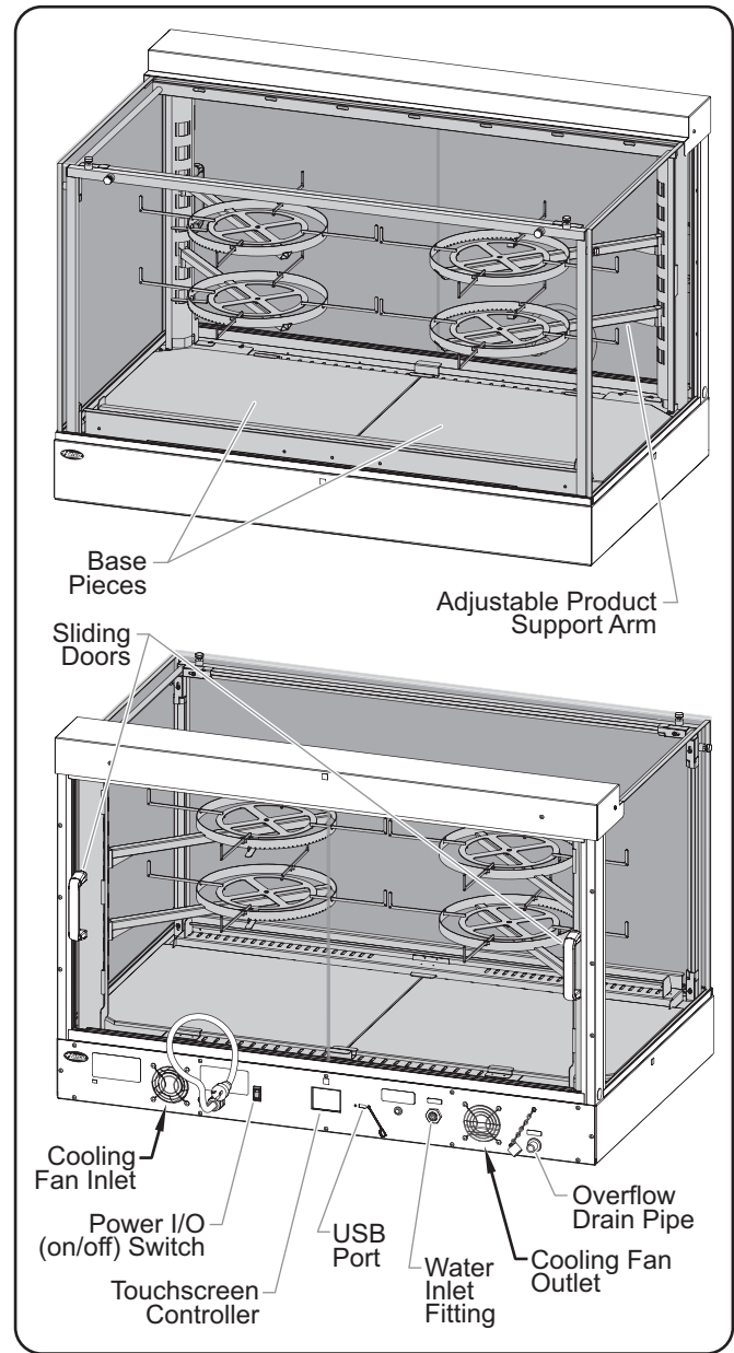
Front and Rear view of Model IHDCH-45
