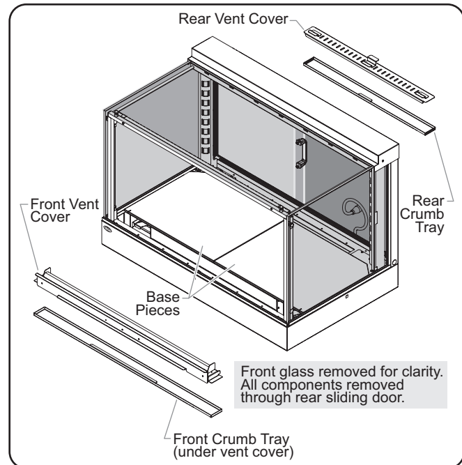
Removing/Installing Components (IHDC-45 shown)
